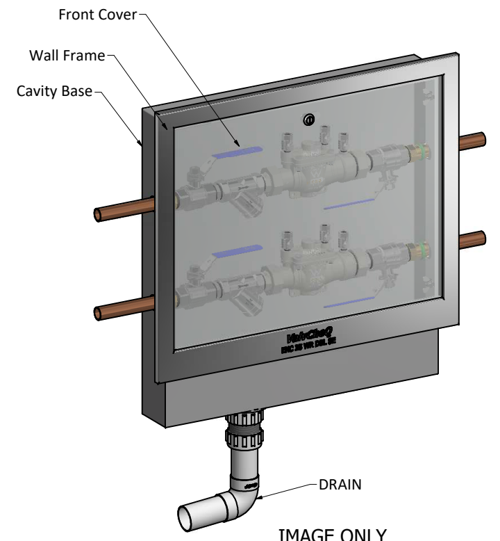
IMAGE ONLY Assembled with Valves Scale ( 1 : 5 )
